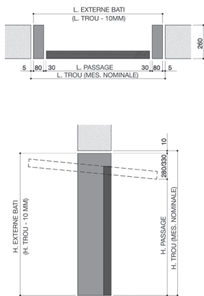
POSITION EN TUNNEL STRUCTURE SPAZIO HF
