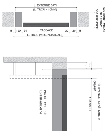
POSITION EN TUNNEL STRUCTURE SIKURA CITY HF
