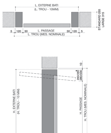
POSITION EN TUNNEL STRUCTURE SIKURTEC HF
