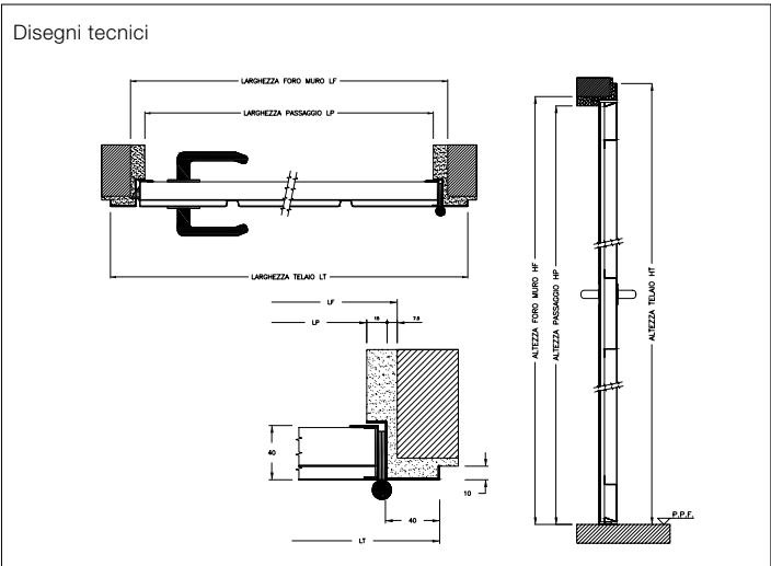
Misure standard porta Pratik
